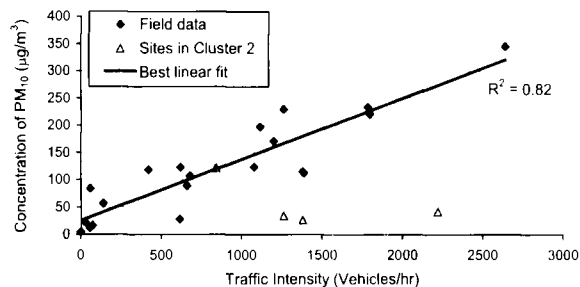
Figure 2: Correlating the PM_{10} concentration to traffic intensity with 20 data, excluding Site 1.1 and Sites 2.1, 2.2, 2.3 and 2.4.
