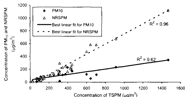
Figure 3: Correlating the concentrations of PM larger than 10\ \mu m (NRSPM) and smaller than 10\ \mu m (i.e. PM_{10} ) to the concentration of TSPM, respectively.
