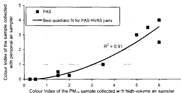
Figure 4: Correlating the colour indices of the SPM samples collected using the personal air samplers, PAS1 and PAS2, with the colour index of the PM_{10} sample collected using the HVAS at 11 sites.
