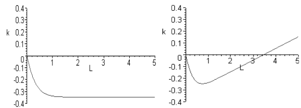
Figure 4: (a) k is \approx -0.38 when \alpha \rightarrow 1 Figure 4: (b) \alpha increased
