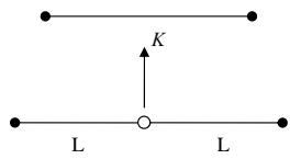
Figure 3: Effective coupling k
