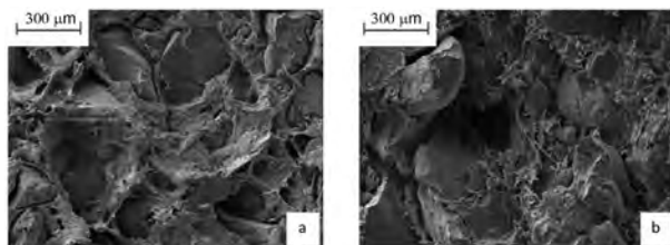
Figure 5: Scanning electron micrographs of tensile fracture surfaces (a) 20GTR/80WPP (b) 80GTR/20WPP
