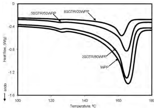
Figure 6: Melting endotherms for WPP and selected blends
