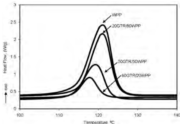
Figure 7: Re-crystallization exotherms for WPP and selected blends
