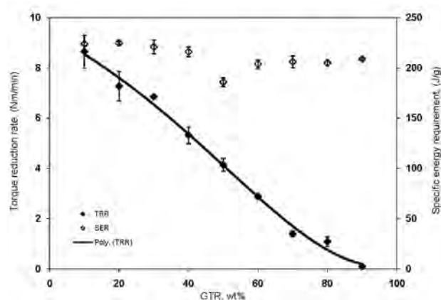
Figure 3: Torque reduction rate and specific energy requirement vs. GTR content
