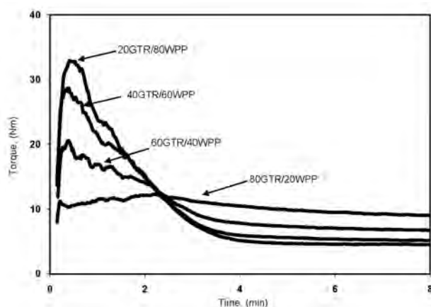
Figure 1: Torque development for GTR, WPP and the 50/50 blend
