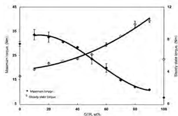
Figure 2: Maximum and steady state torque vs. GTR content
