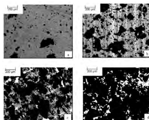
Figure 4: Optical Micrographs ( \times 10 )
