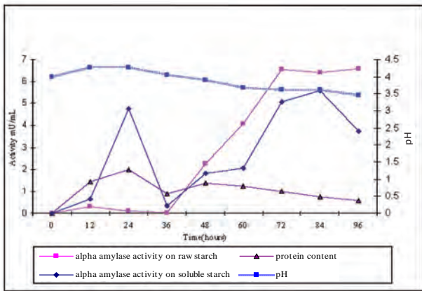
Figure 5: \alpha -amylase activity, pH and protein content of the culture supernatant of Geotrichum spp.
