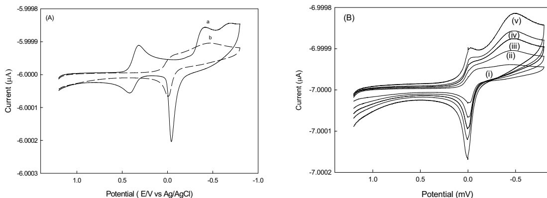
Figure 4: (A) Combined cyclic voltammograms of (a) 200 ppm Cu(II)-nitrate and (b) 200 ppm Cu-sac-phen complex at scan rate 100 \text{ mVs}^{-1} and (B) Cyclic voltammograms of Cu-sac-phen complex (200 ppm) at different scan rate: i) 50, ii) 100, iii) 150 and iv) 200 \text{mVs}^{-1} in 0.1M KCl
