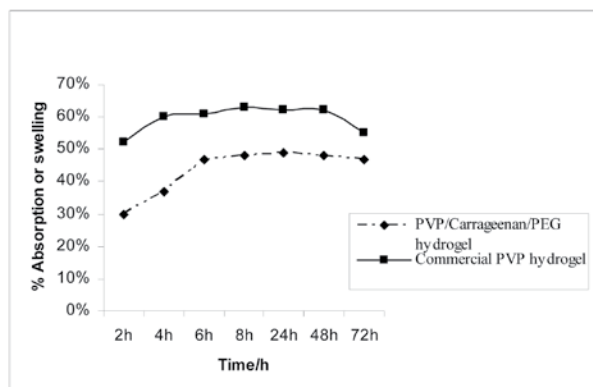
Figure 3: Absorption behaviour of PVP/Carr/PEG hydrogel in PECF compared to the commercial PVP hydrogel
