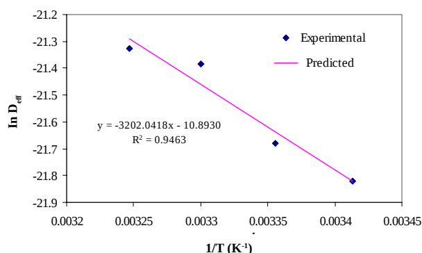
Figure 5: The relationship between \ln D_{eff} and 1/T of drying
