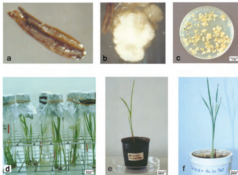
Figure 1: Anther culture response of indica × japonica crosses
