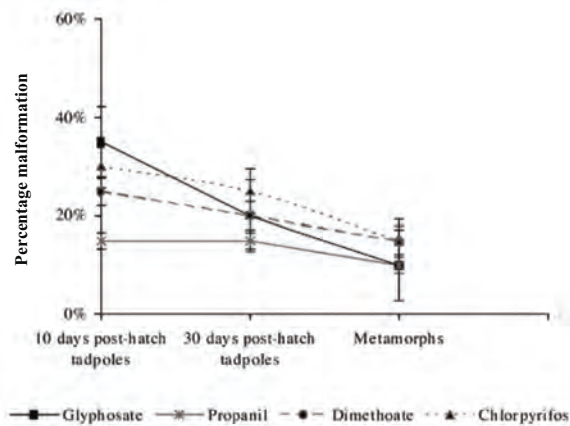
Figure 4: Percentage incidence of malformations at 10 days and 30 days post-hatch tadpoles and metamorphs of B. melanostictus exposed to the highest concentration of the pesticide (0.5 ppm for chlorpyrifos and 1.0 ppm for dimethoate, glyphosate and propanil). The percentage malformation was calculated as the number of abnormal individuals (including the dead abnormal ones) at a given age divided by the initial number of tadpoles.
