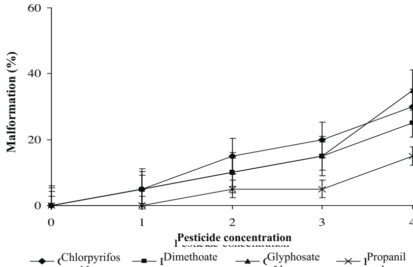
Figure 2: Percentage incidence of malformation observed in 10 days post-hatch tadpoles of B. melanostictus exposed to different concentrations of the four pesticides. 0 = control, 1 - 4 denotes the increasing order of the pesticide dose (1 = 0.05 ppm, 2 = 0.1 ppm, 3 = 0.25 ppm and 4 = 0.5 ppm for chlorpyrifos, and 1 = 0.25 ppm, 2 = 0.5 ppm, 3 = 0.75 ppm and 4 = 1.0 ppm for other pesticides).
