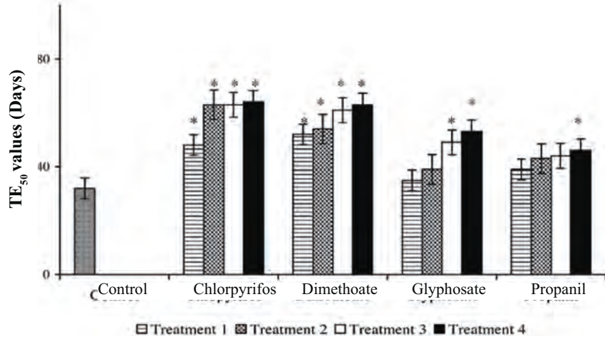
Figure 1: Average TE 50 (time required for forelimb emergence in half the number of tadpoles) values of tadpoles of B. melanostictus exposed to chlorpyrifos, dimethoate, glyphosate and propanil at different concentrations (exposure levels are given as Treatment 1 = 0.05 ppm, 2 = 0.10 ppm, 3 = 0.25 ppm and 4 = 0.5 ppm for chlorpyrifos, and Treatment 1 = 0.25 ppm, 2 = 0.50 ppm, 3 = 0.75 ppm and 4 = 1.0 ppm for other chemicals). *Represents the TE 50 values significant at p < 0.05 (ANOVA) compared to the control
