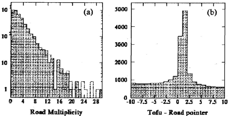
Figure 2: (a) Multiplicity of tracks found by the tracking trigger hardware during the 1994 run. (b) Correspondence between the track pointers and TOFU counters containing actual hits.
