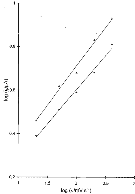
Figure 3: A plot of \log (i_p/\mu\text{A}) vs. \log (v/\text{mV s}^{-1}) for 1.0 \times 10^{-3} \text{ mol dm}^{-3} Paracetamol solution in 0.1 \text{ mol dm}^{-3} \text{ NaCl} at (▲) bare (◆) HDMS modified GC electrode.
