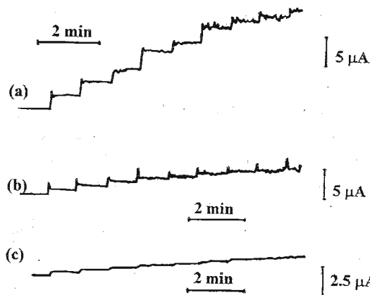
Figure 4: Amperometric responses at the HDMS modified electrode under \text{N}_2 saturated (a) Paracetamol at +0.55 \text{ V} (b) Ascorbic acid at +0.40 \text{ V} (c) Catechol at +0.55 \text{ V} . Supporting electrolyte 0.1 \text{ mol dm}^{-3} \text{ NaCl} .
