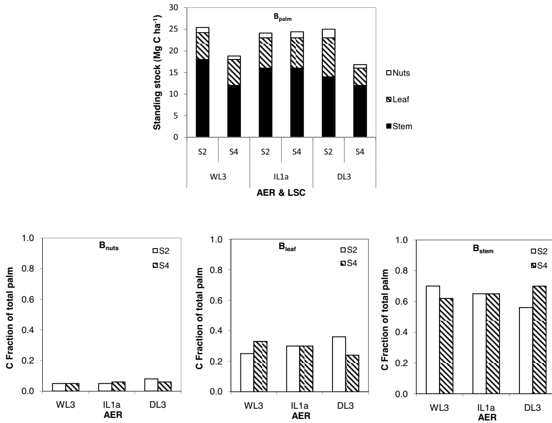
Figure 1: C stock of the whole palm ( B_{palm} ) ( Mg\ C\ ha^{-1} ) in terms of its components (stem, leaf, nuts), and the fraction of C in different components; nuts ( B_{nut} ), leaves ( B_{leaf} ) and stem ( B_{stem} ) on S_2 and S_4 land suitability classes in WL_3 , IL_{1a} and DL_3 .
