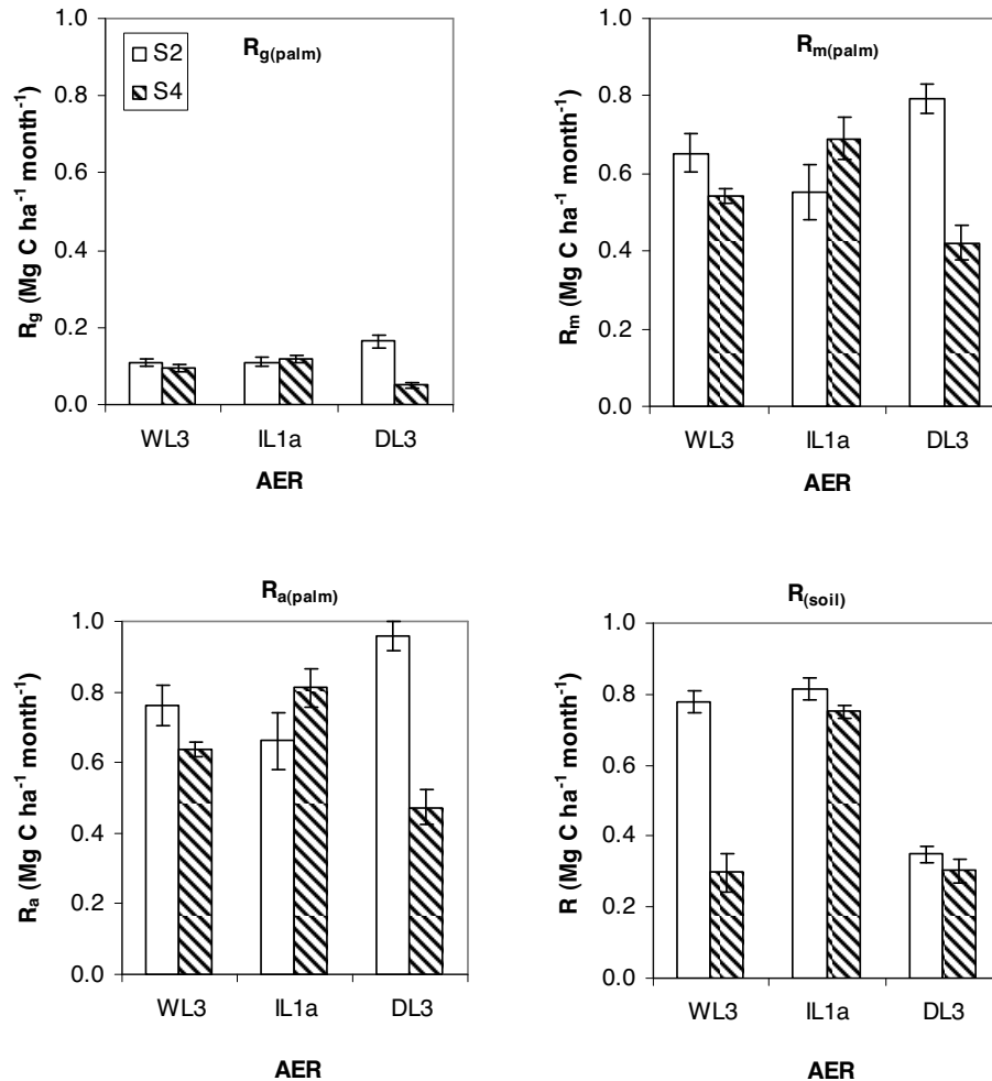
Figure 6a: Growth Respiration, [ R_{g(palm)} ] (Mg C ha -1 month -1 ), maintenance respiration [ R_{m(palm)} ] and total respiration [ R_{a(palm)} ] of coconut palms and soil respiration [ R_{(soil)} ] on S_2 and S_4 land suitability classes in WL_3 , IL_{1a} and DL_3 (values are means \pm standard error of mean).
