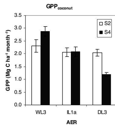
Figure 4: Gross Primary Production (GPP) of coconut palms ( \text{Mg C ha}^{-1} \text{ month}^{-1} ) on S_2 and S_4 land suitability classes in WL_3 , IL_{1a} and DL_3 (values are means \pm standard error of mean)
