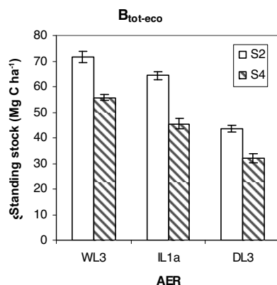
Figure 3: C stock ( \text{Mg C ha}^{-1} ) of the total ecosystem ( B_{tot-eco} ) on S_2 and S_4 land suitability classes in WL_3 , IL_{1a} and DL_3 (values are means \pm standard error of mean)
