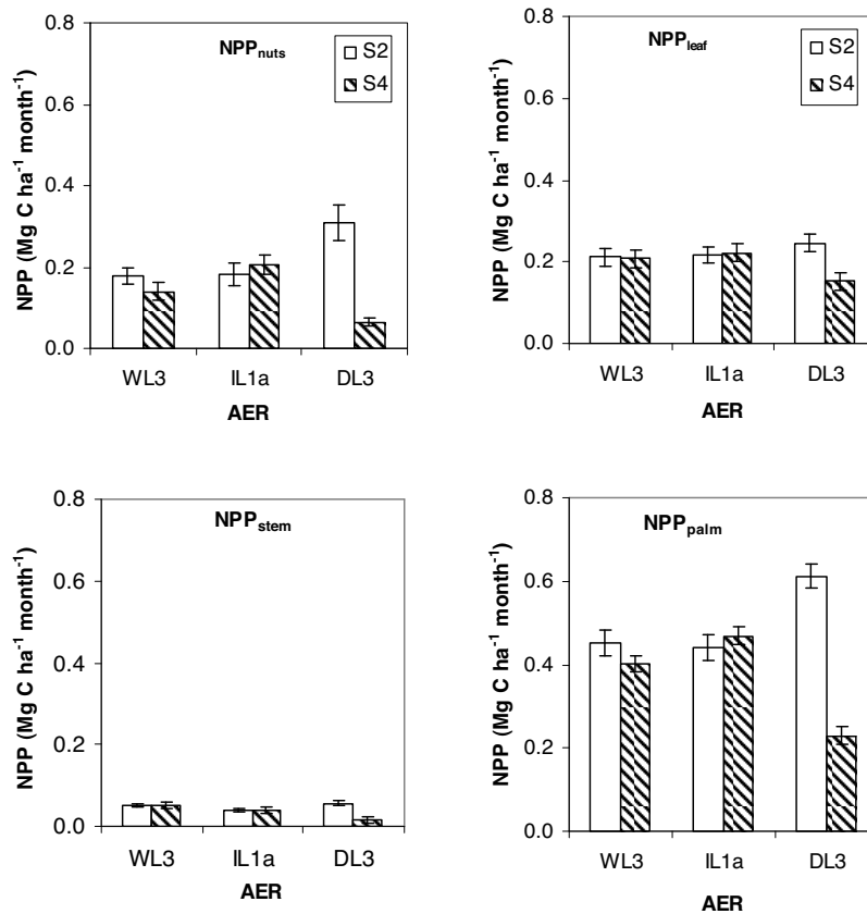
Figure 5: Net Primary Production ( \text{Mg C ha}^{-1} \text{ month}^{-1} ) of nuts ( NPP_{nut} ), leaves ( NPP_{leaf} ), stem ( NPP_{stem} ) and total coconut palm ( NPP_{palm} ) on S_2 and S_4 land suitability classes in WL_3 , IL_{1a} and DL_3 (values are means \pm standard error of mean)
