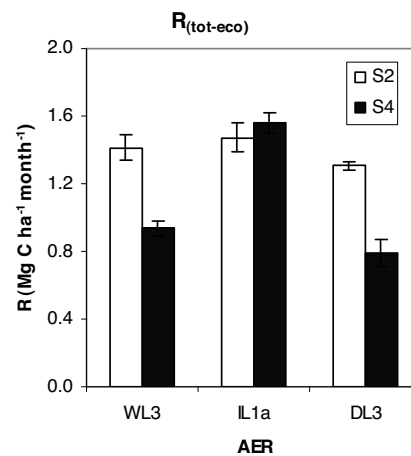
Figure 6b: Total ecosystem respiration [ R_{(tot-eco)} ] on S_2 and S_4 land suitability classes in WL_3 , IL_{1a} and DL_3
