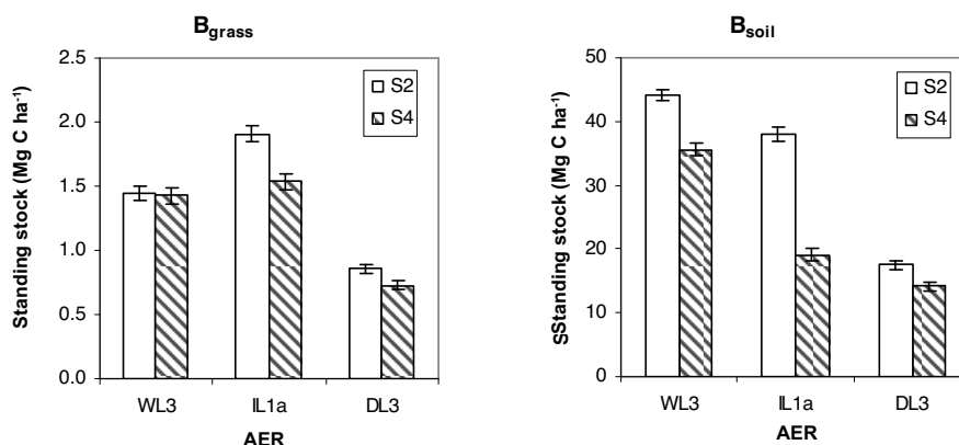
Figure 2: C stock (Mg C ha -1 ) of grass cover ( B_{grass} ) and top soil ( B_{soil} ) on S_2 and S_4 land suitability classes in WL_3 , IL_{1a} and DL_3 (values are means \pm standard error of mean)
