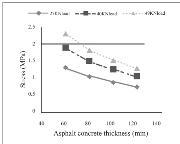
Figure 9: Maximum principal stress variation with asphalt concrete thickness
