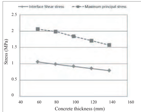
Figure 7: Stress variation with concrete thickness
