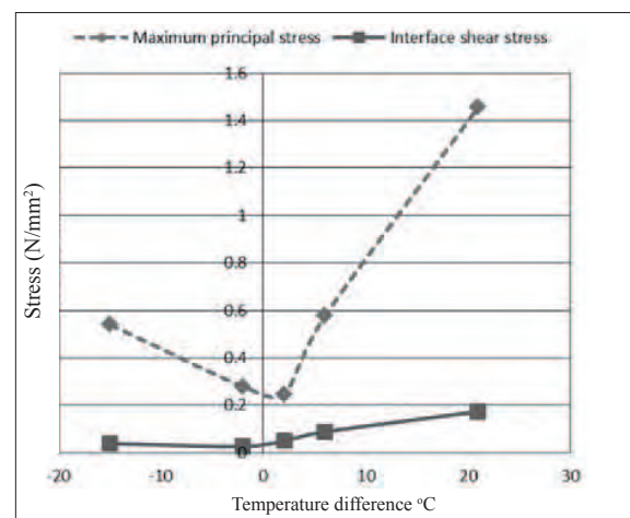
Figure 5: Stresses variation with temperature difference
