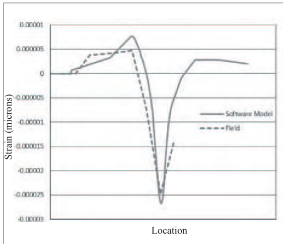
Figure 2: Strains induced at gauge location 1 (top)
