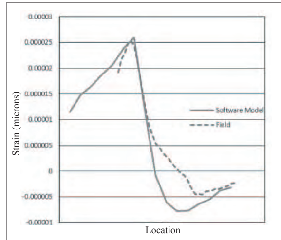
Figure 3: Verification of strains at gauge location 2 (bottom)
