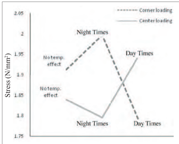
Figure 6: Stresses variation with temperature and loading position
