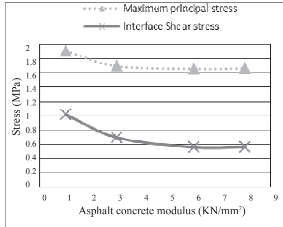
b) Asphalt elastic modulus
