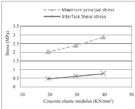
a) Concrete elastic modulus
