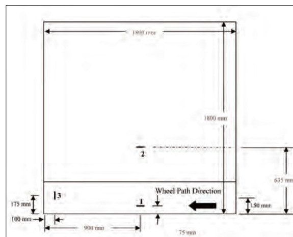
Figure 1: Strain gauge locations
