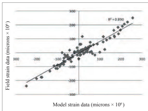
Figure 4: Correlation between model strain data and the field strain data
