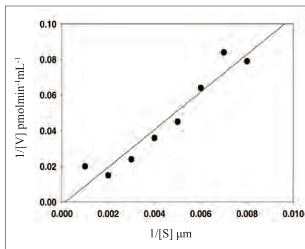
Figure 5: Lineweaver-Burk plot of the purified protease activity at pH 9.0 and 40 °C using different concentrations of substrate
