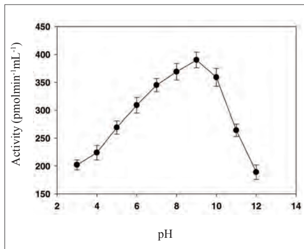
Figure 2: Effect of pH on protease activity of purified enzyme
