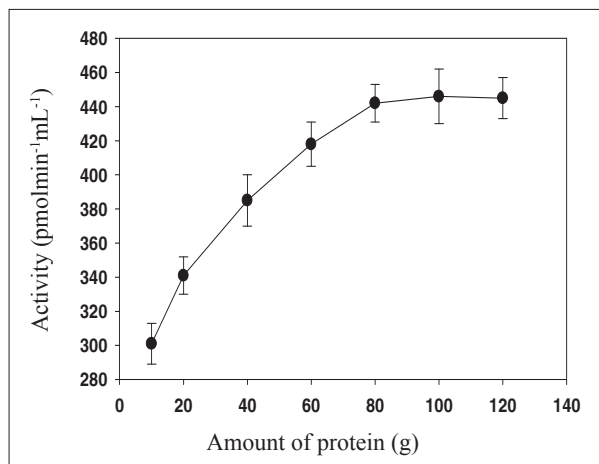
Figure 4: Effect of enzyme concentration on the purified protease activity
