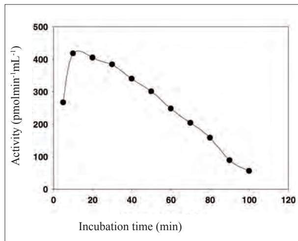
Figure 1: Effect of time of incubation on protease activity of 70 % ammonium sulfate precipitated extract
