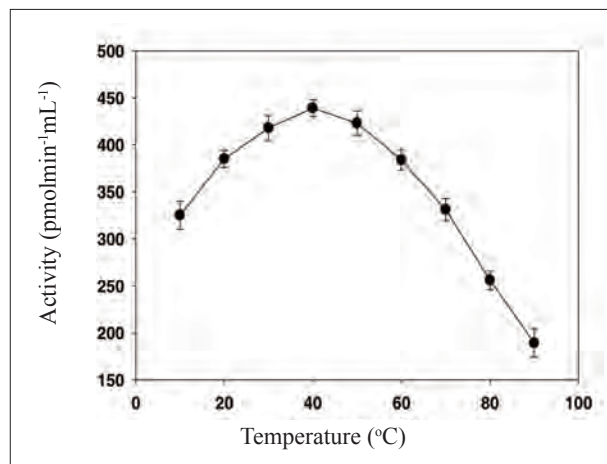
Figure 3: Effect of temperature on the purified protease activity
