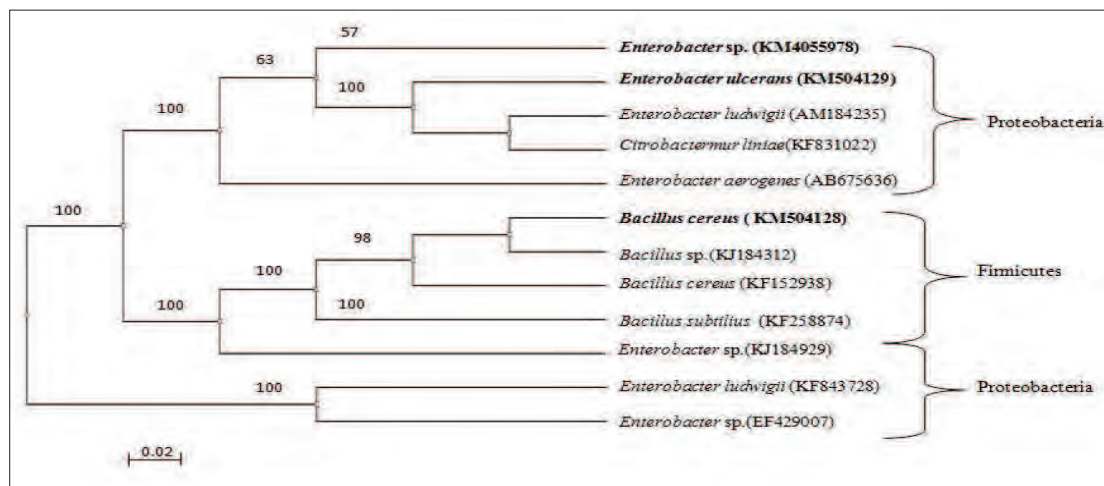
Figure 4: Phylogenetic relationship based on 16S rRNA sequences and the most closely related hydrocarbon degraders recorded, which are found from NCBI.
