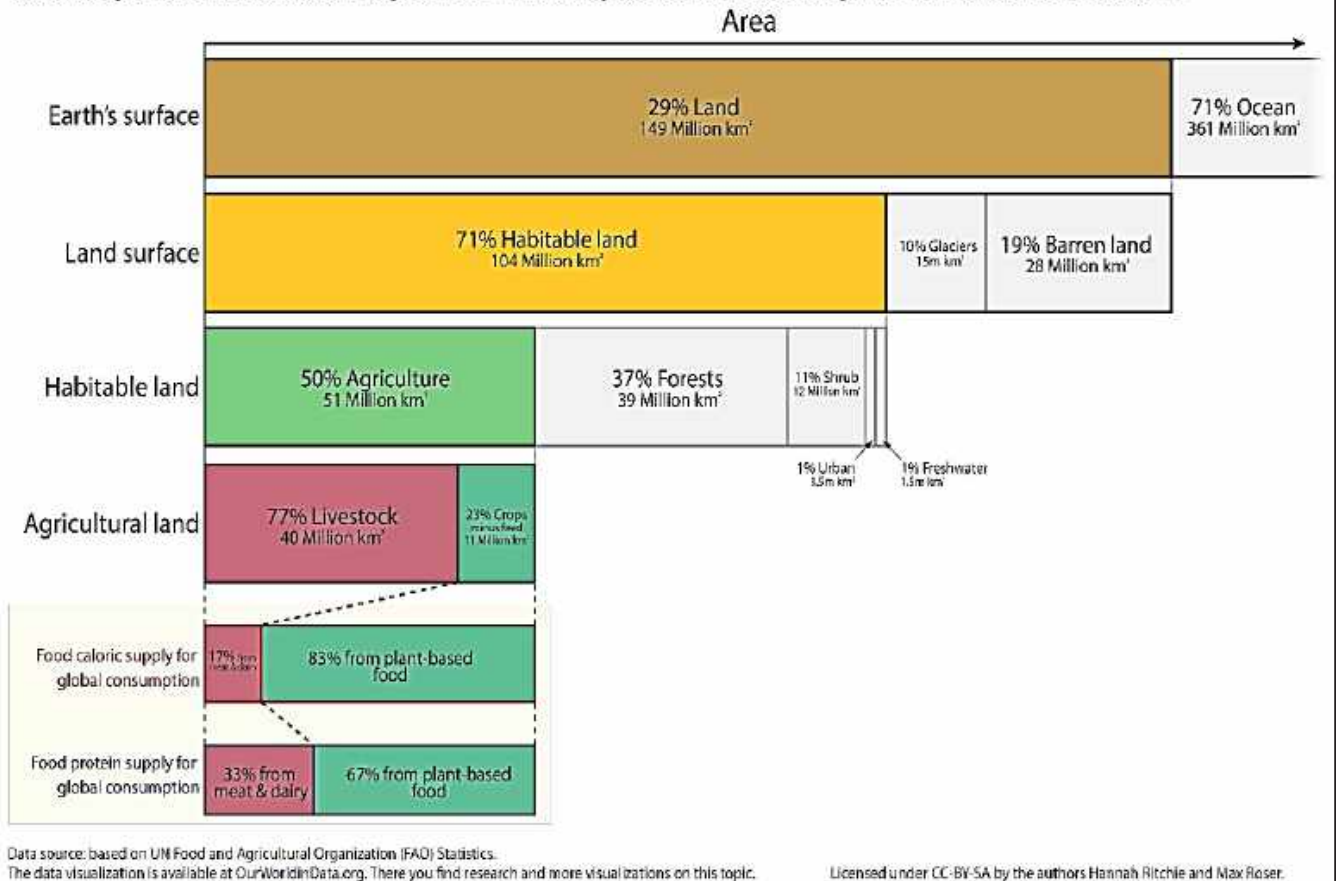
Fig 2 : Distribution of Earth's land resources
