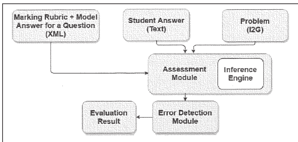
Fig 5 : System to assess Geometric theorem proving questions
